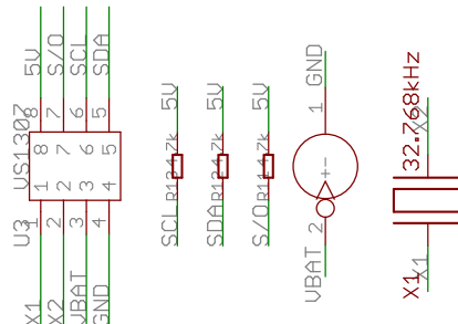
RTC
